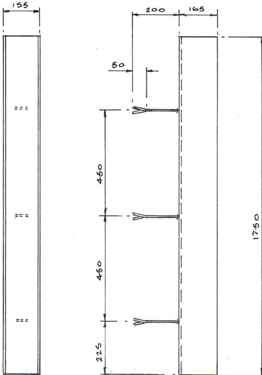
SIDE ELEVATION 1:10
